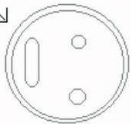
eoplast
